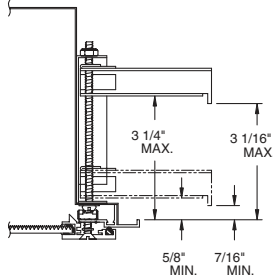
T-BAR BRACKET DETAIL
