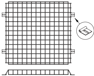
FLANGE SWING BAR DETAIL
